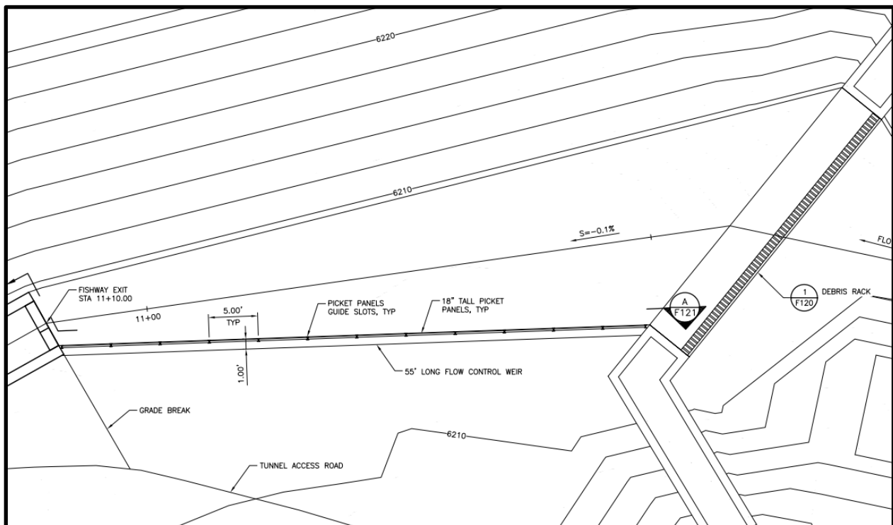
Figure 2-5. Overhead view of the flow control weir located between the debris rack and fishway
